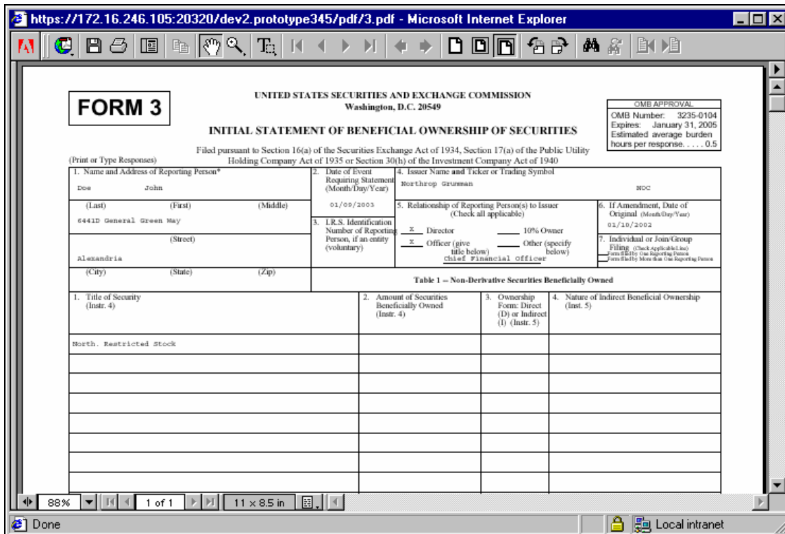
Figure 8-23: PDF Document
