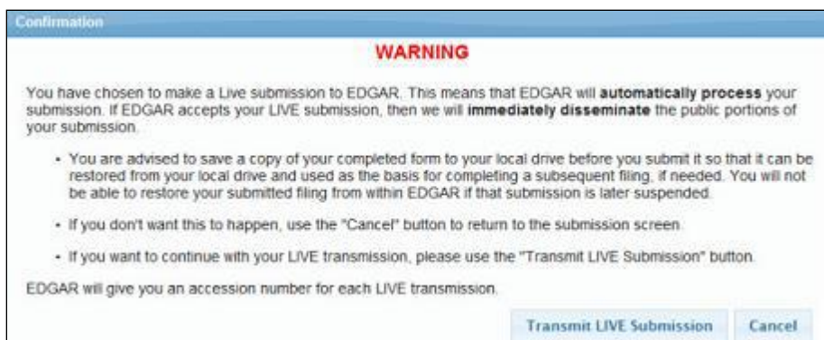
Figure 8-191: Confirmation/Warning screen
