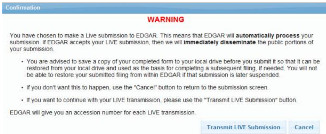
Figure 8-276: Confirmation Screen
