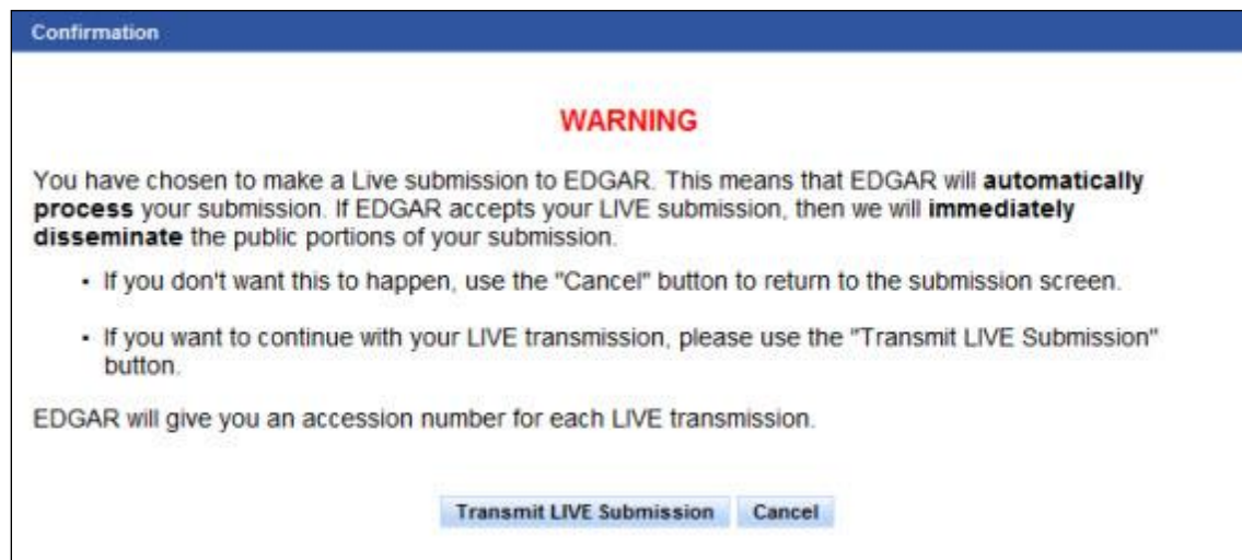
Figure 8-124: Confirmation Screen
