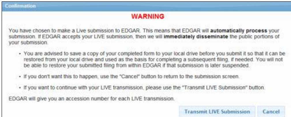
Figure 8-77: Confirmation/Warning Screen
