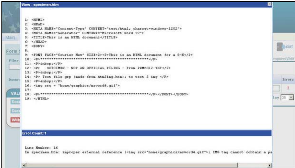
Figure 7-36: Document Validation Window
