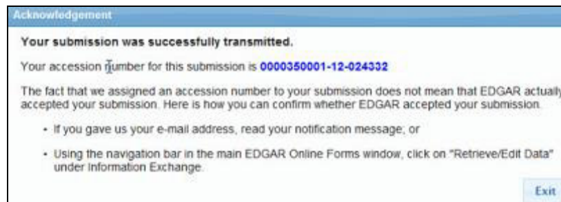
Figure 9-92: Acknowledgment screen
