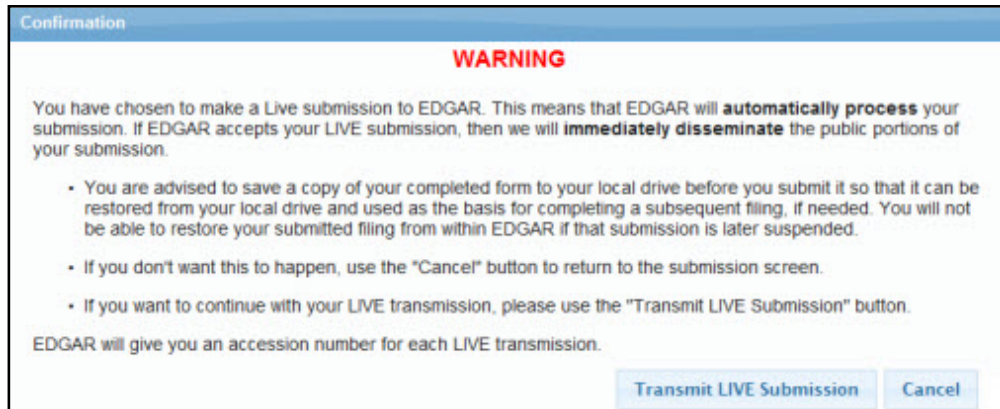
Figure 9-77: Confirmation/Warning Screen
