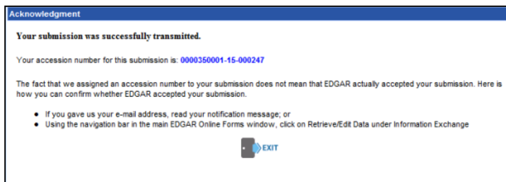
Figure 9-118: Acknowledgment Screen
