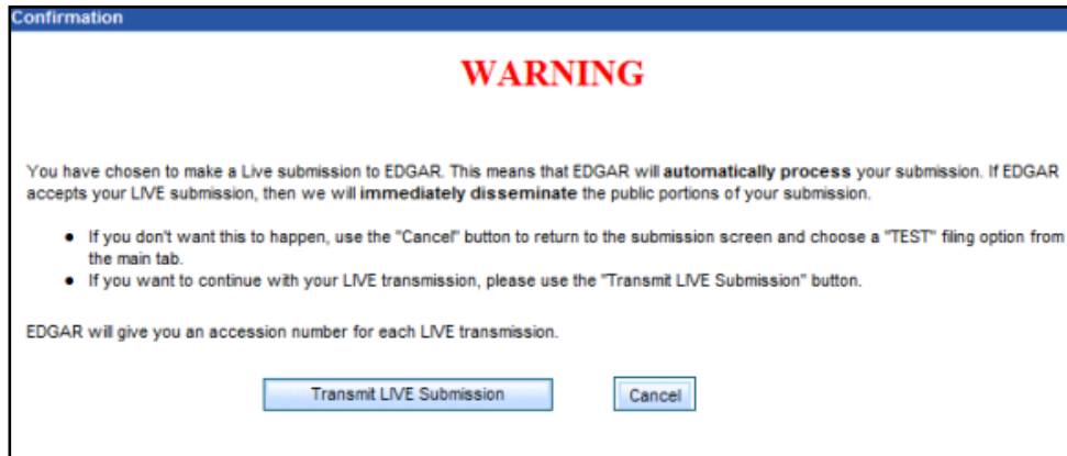
Figure 9-117: Confirmation Screen
