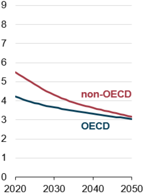
Energy intensity thousand British thermal units per 2015 dollar of GDP
