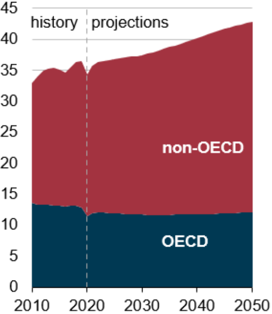
Energy-related CO 2 emissions billion metric tons
