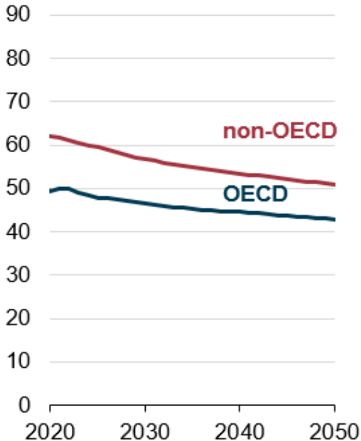
Carbon intensity metric tons CO 2 per billion British thermal units
