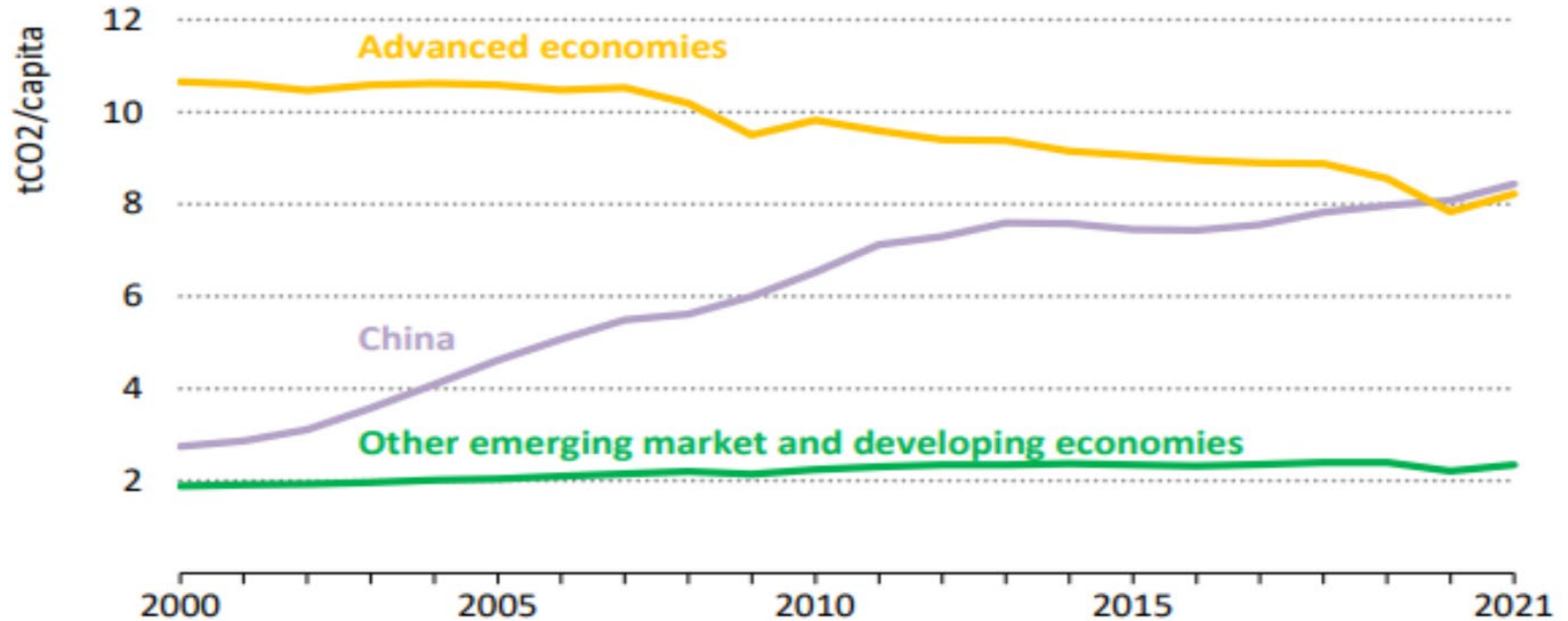
Figure 6 CO2 emissions per capita by region, 2000-2021
