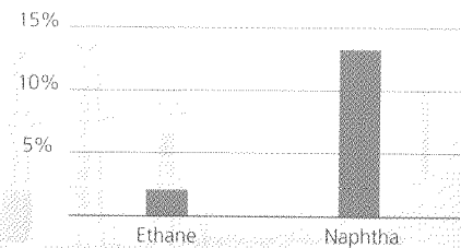
Butadiene/Ethylene Production Yield
