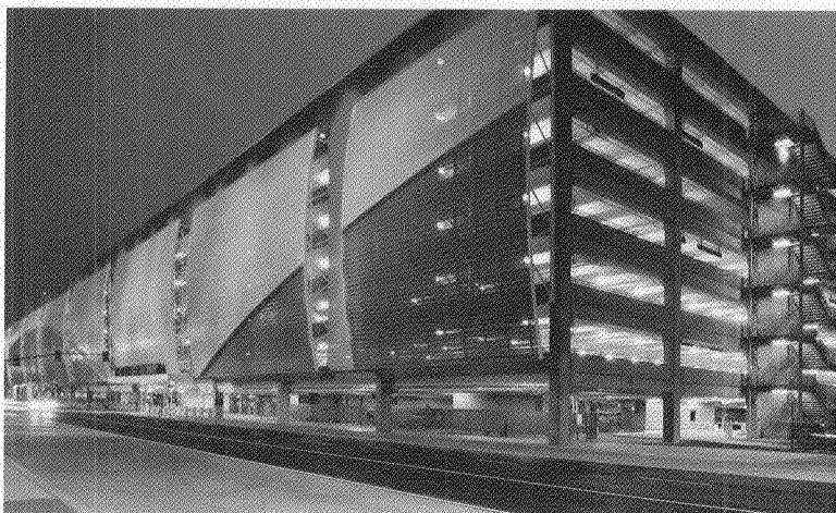
The eight-level structure contains 3,817 precast concrete components and is the largest precast concrete parking structure in the state of California, providing spaces for 3,350 cars.
