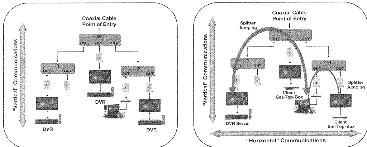
In-home coaxial cable architecture designed for "vertical" communications creates "islands" of digital entertainment
