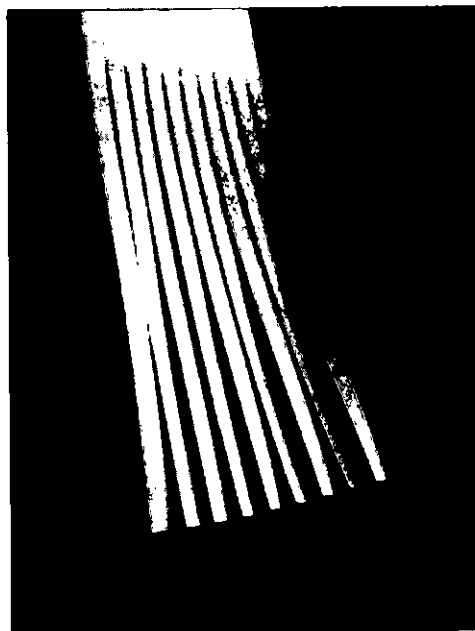
Multiple, ribbon-shaped HTS wires with industry-standard dimensions can be produced after first producing coatings on a wider strip. Shown is a partially slit 4 cm wide strip.
