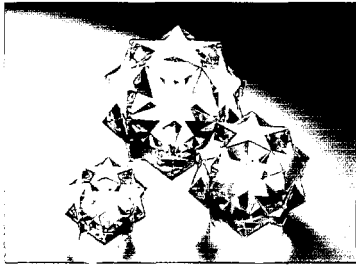
Constellation
