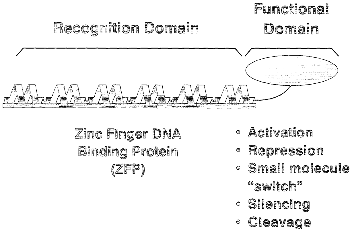
Figure A: The two domain structure of a ZFP TF
