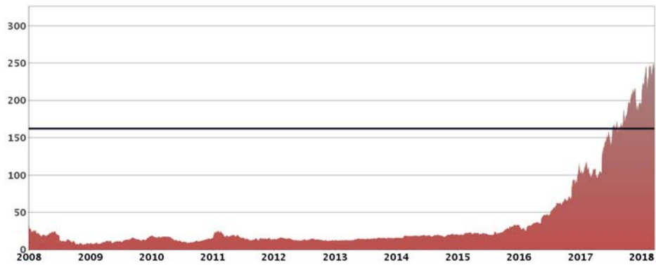
NVIDIA Corporation – Daily Closing Prices January 1, 2008 to March 20, 2018
