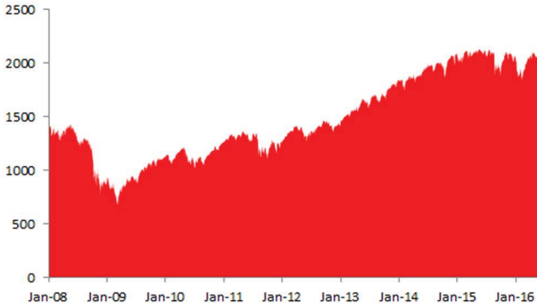
Historical Performance of the Underlying Index – Daily Official Closing Levels January 2, 2008 to June 17, 2016
