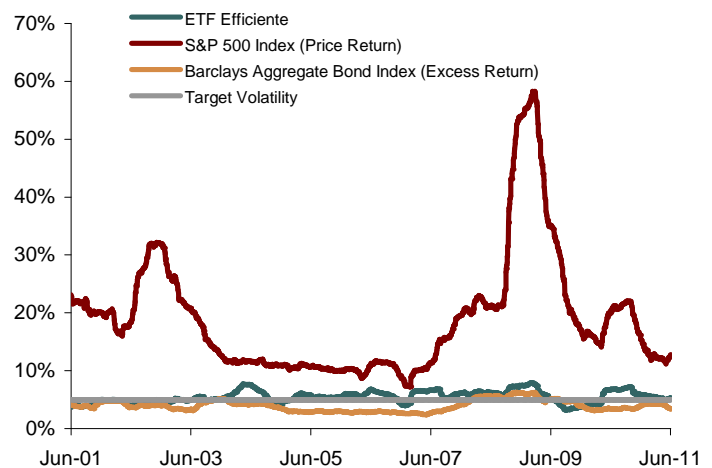
Hypothetical and Actual Historical Volatility – June 29, 2001 to June 30, 2011
