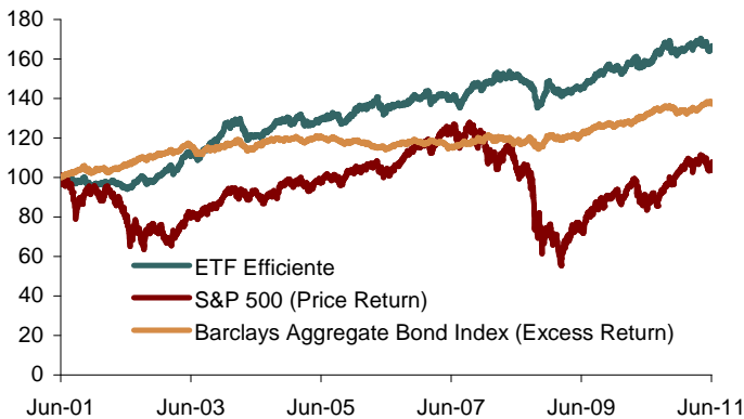
Hypothetical and Actual Historical Performance - June 29, 2001 to June 30, 2011
