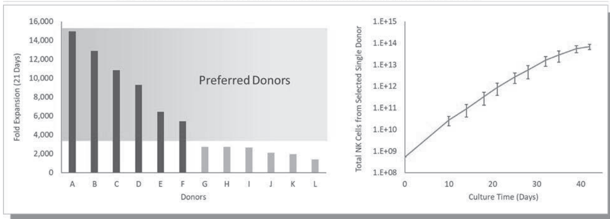
NK CELL DONOR SELECTION TO SUPPORT ROBUST CELL EXPANSION
