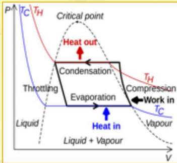
Carnot Cycle
