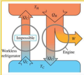
2 nd Law Thermodynamics
