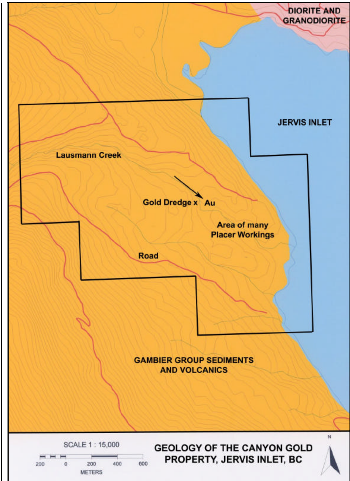
Fig. 5 GEOLOGY OF THE CANYON GOLD PROPERTY
