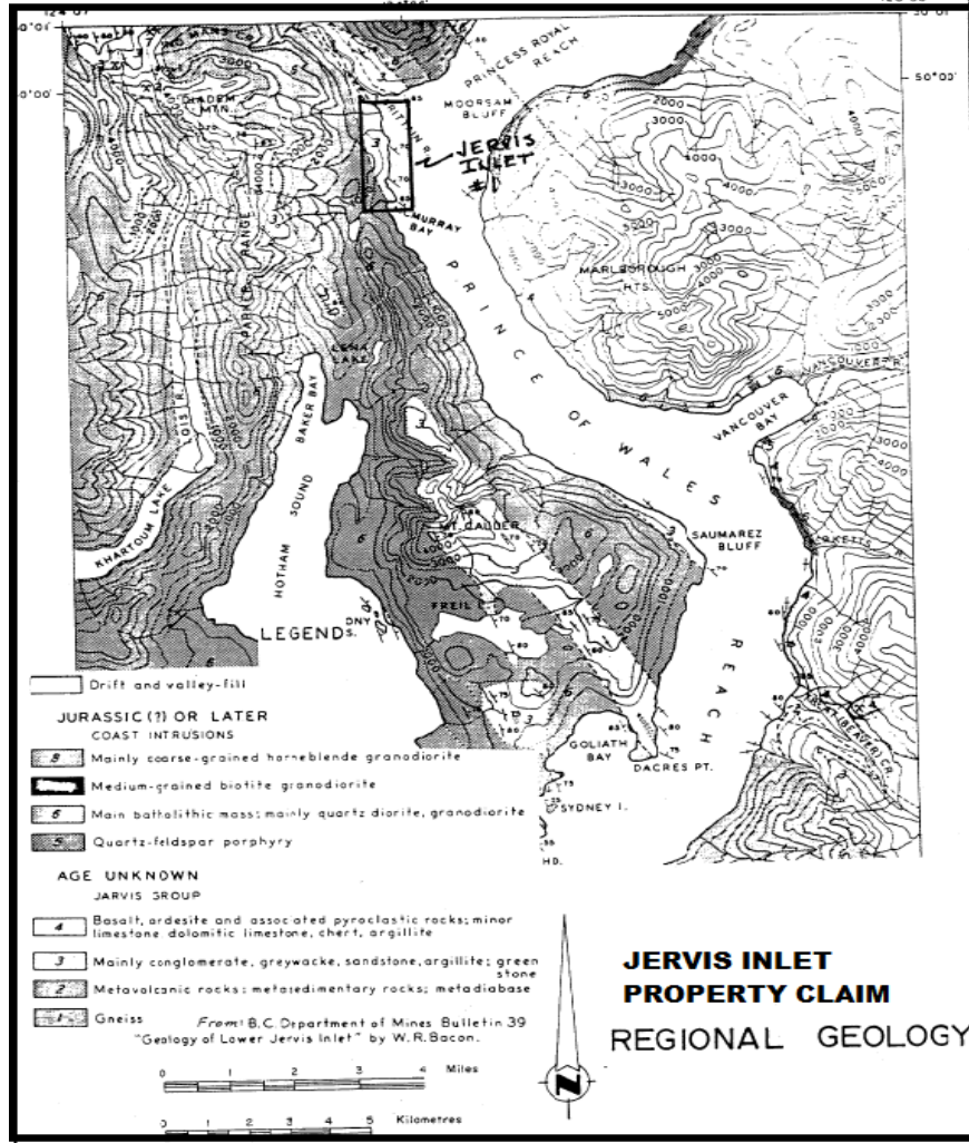
Fig. 4 REGIONAL GEOLOGY MAP OF THE JERVIS INLET AREA
