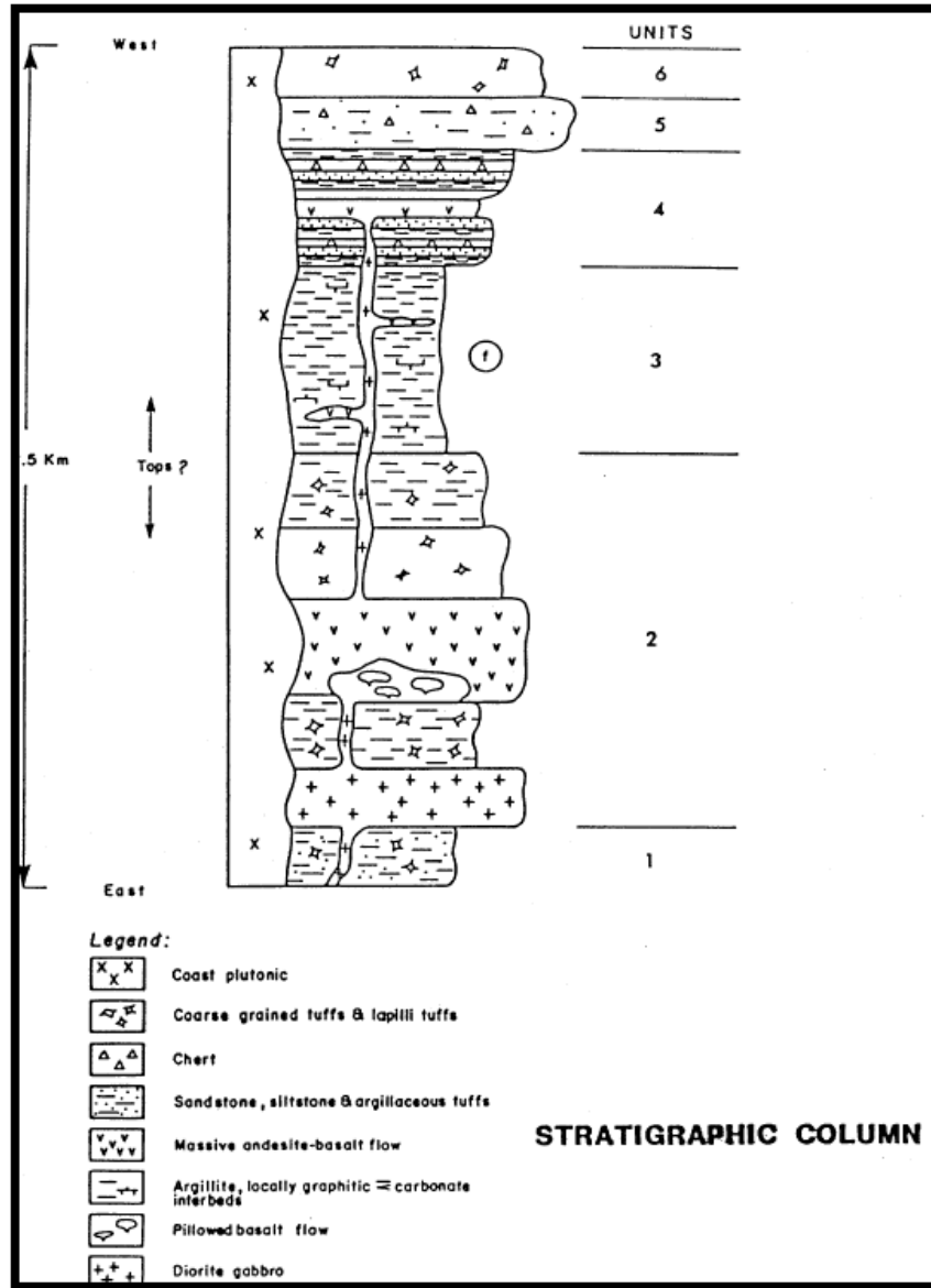
Fig. 6 STRATIGRAPHIC COLUMN OF THE JERVIS INLET AREA
