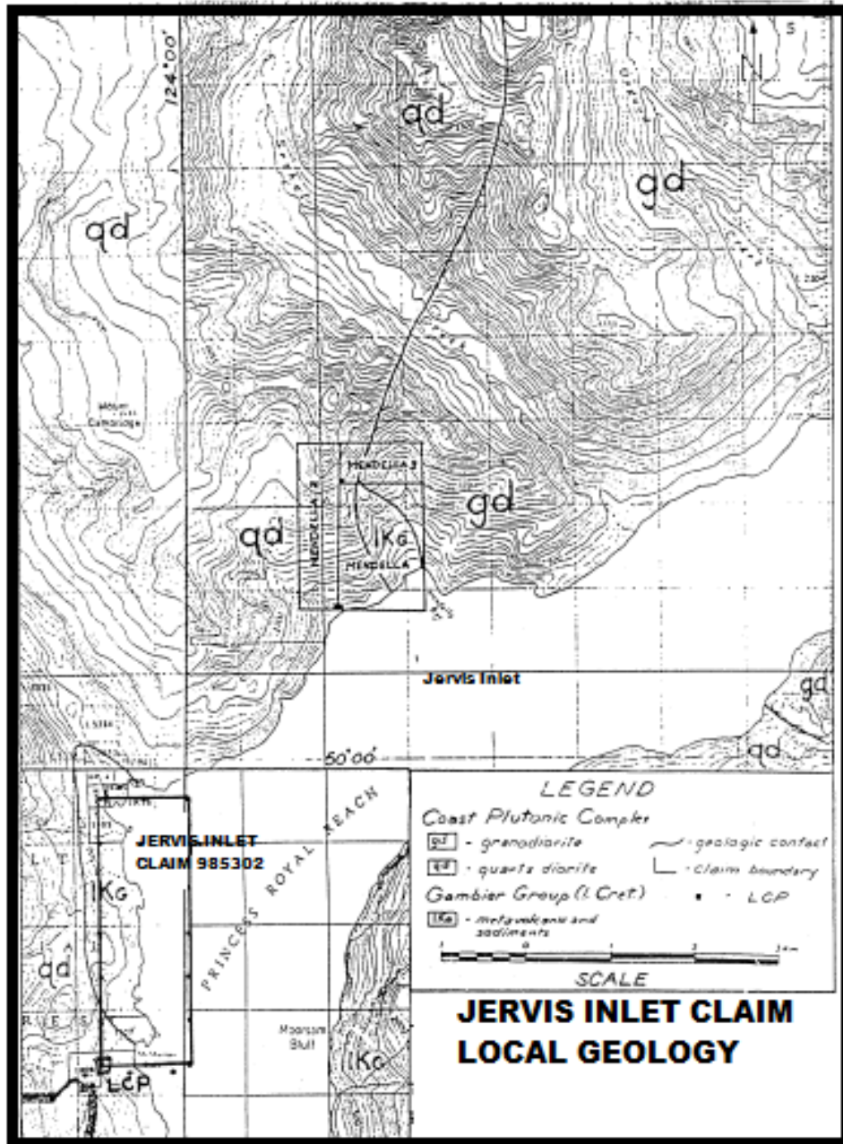
Fig. 5 LOCAL GEOLOGY MAP OF THE JERVIS INLET CLAIM
