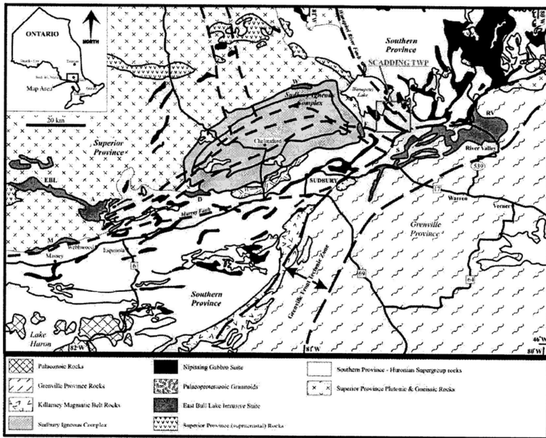
Figure 1. Location of Scadding Township in the Sudbury Mining Division, north-central Ontario, Canada.
